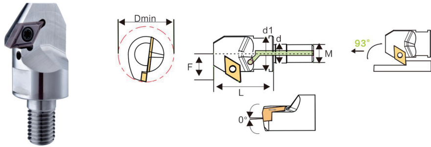
Modular Cutter Head CSA-M-SDZCR series
