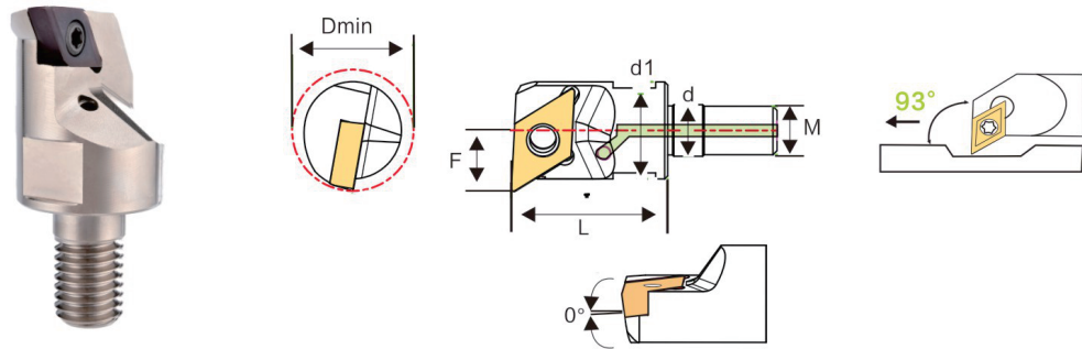
Modular Cutter Head CSA-M-SDUCR series
