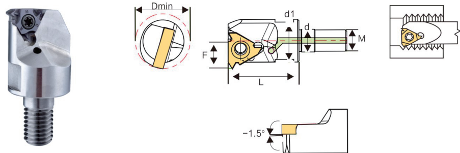
Modular Cutter Head CSA-M-SNR series
