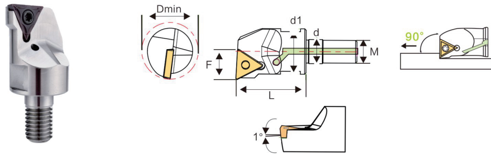
Modular Cutter Head CSA-M-STUCR series
